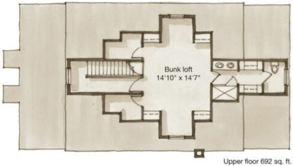
Floor Plan - 2nd Floor
