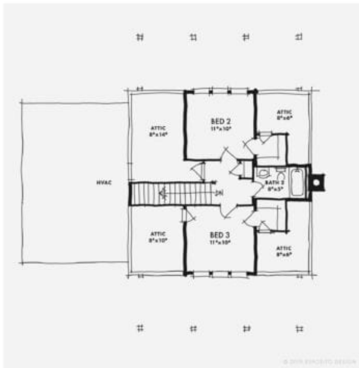
Floor Plan - 2nd Floor
