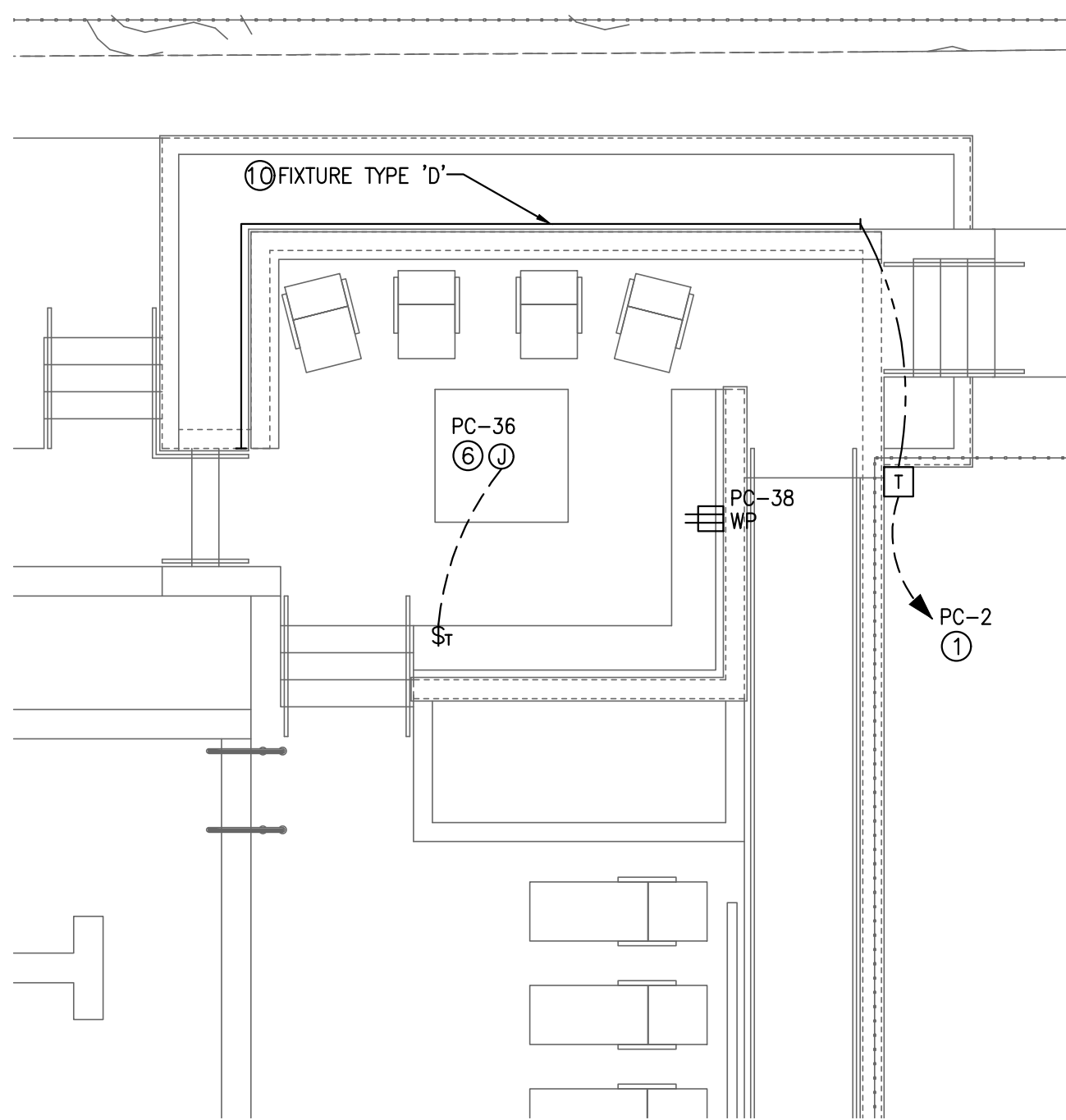
ENLARGED FIRE PIT AREA SCALE 3/16"=1'-0"
