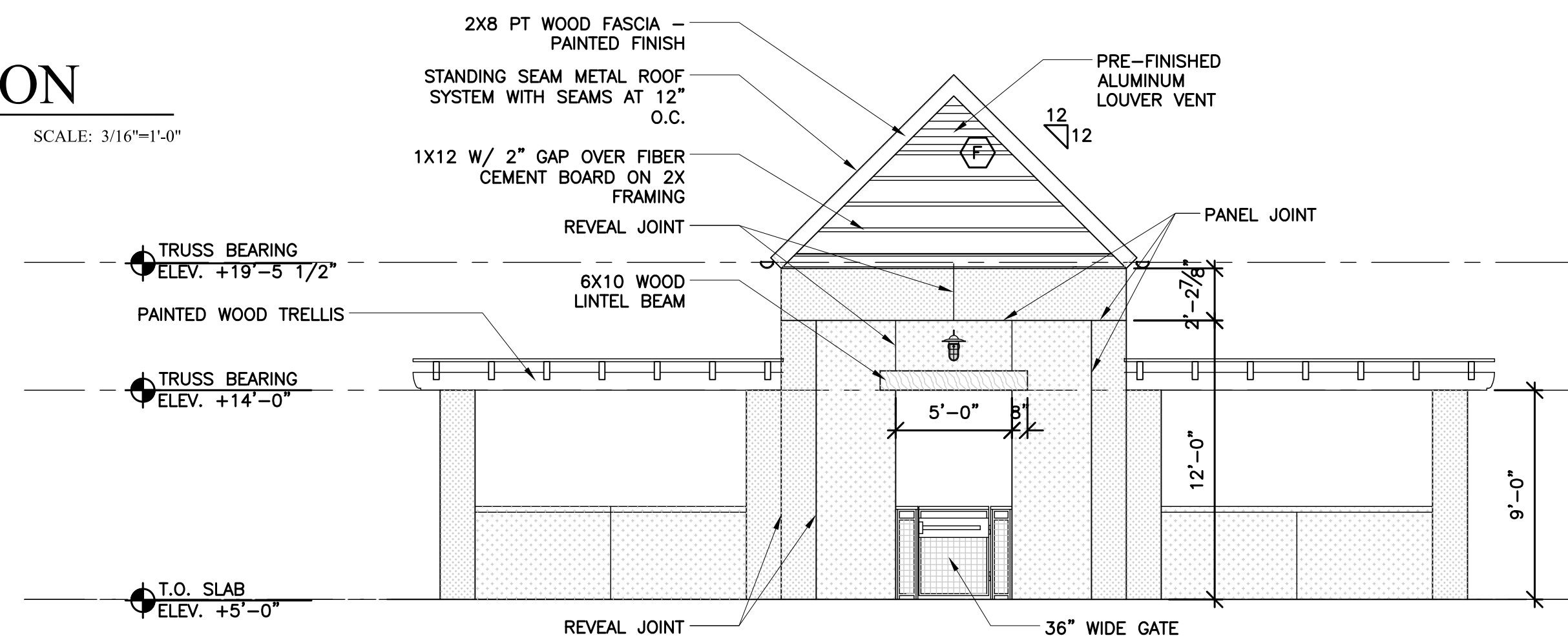
4 POOL GRILLE POOL ELEVATION SCALE: 3/16"=1'-0"
