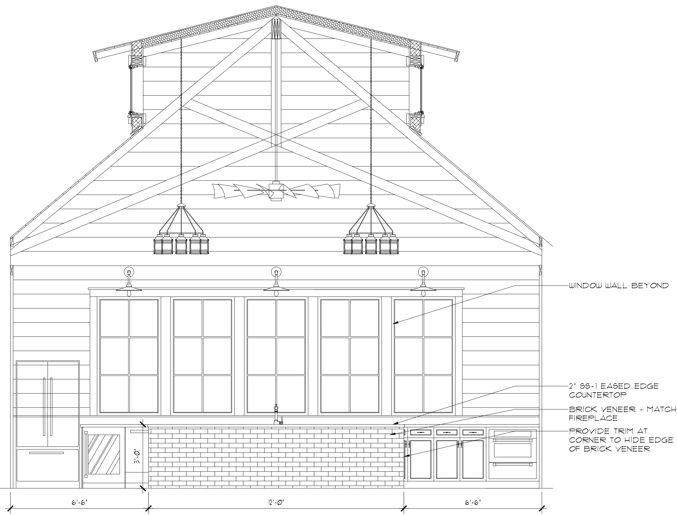
4 RM 102 - EAST WALL SCALE: 3/8" = 1'-0"
