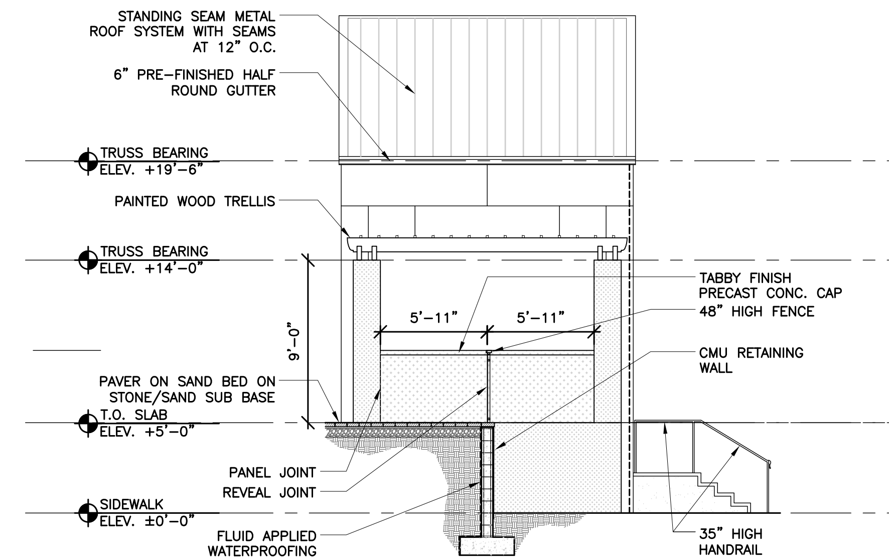
3 POOL GRILLE SIDE ELEVATION SCALE: 3/16"=1'-0"
