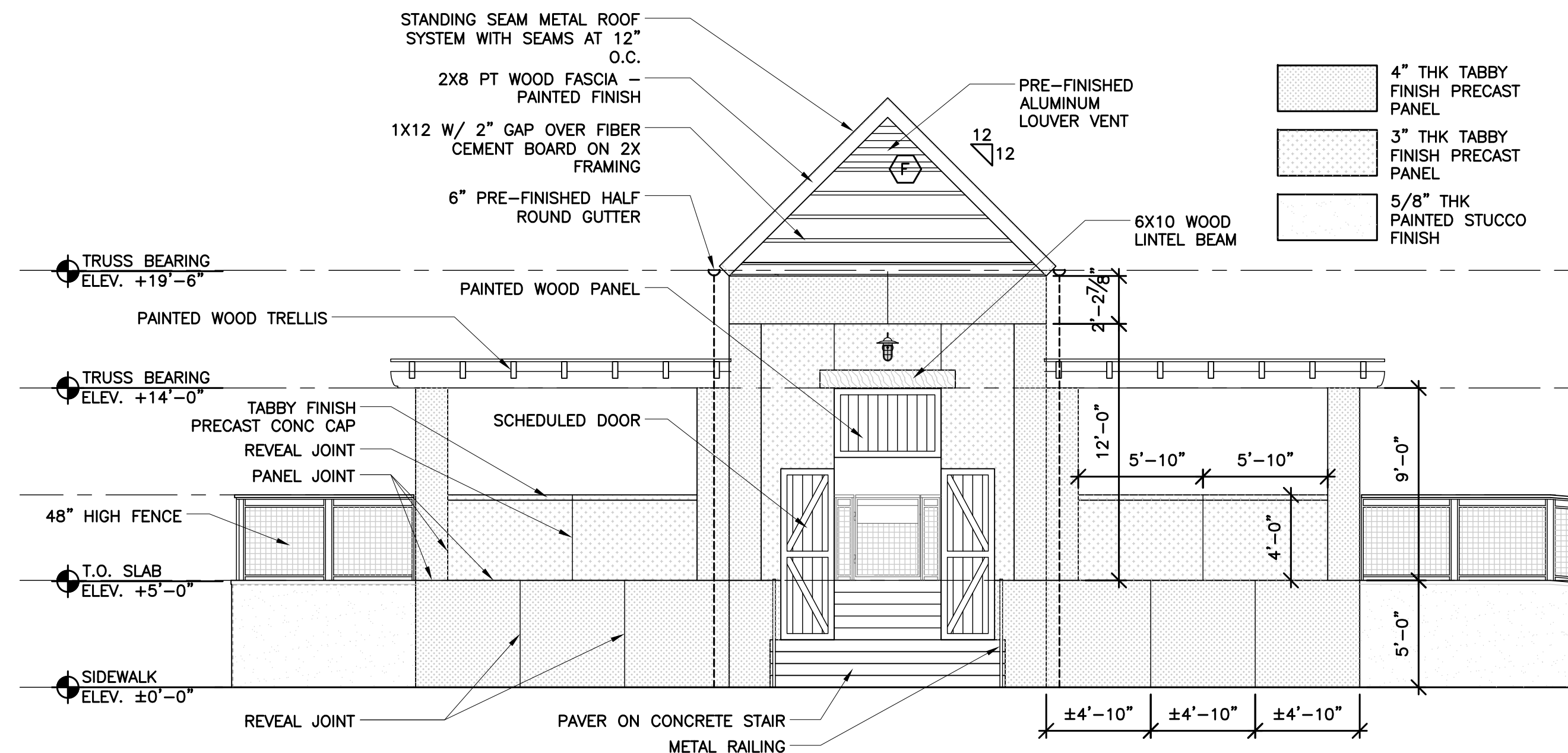
2 POOL GRILLE ENTRY ELEVATION SCALE: 3/16"=1'-0"
