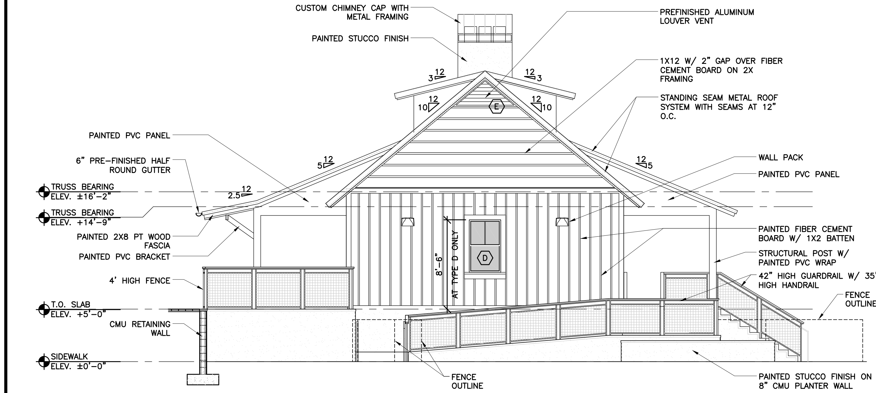
2 CLUBHOUSE RIGHT SIDE ELEVATION SCALE: 3/16"=1'-0"
