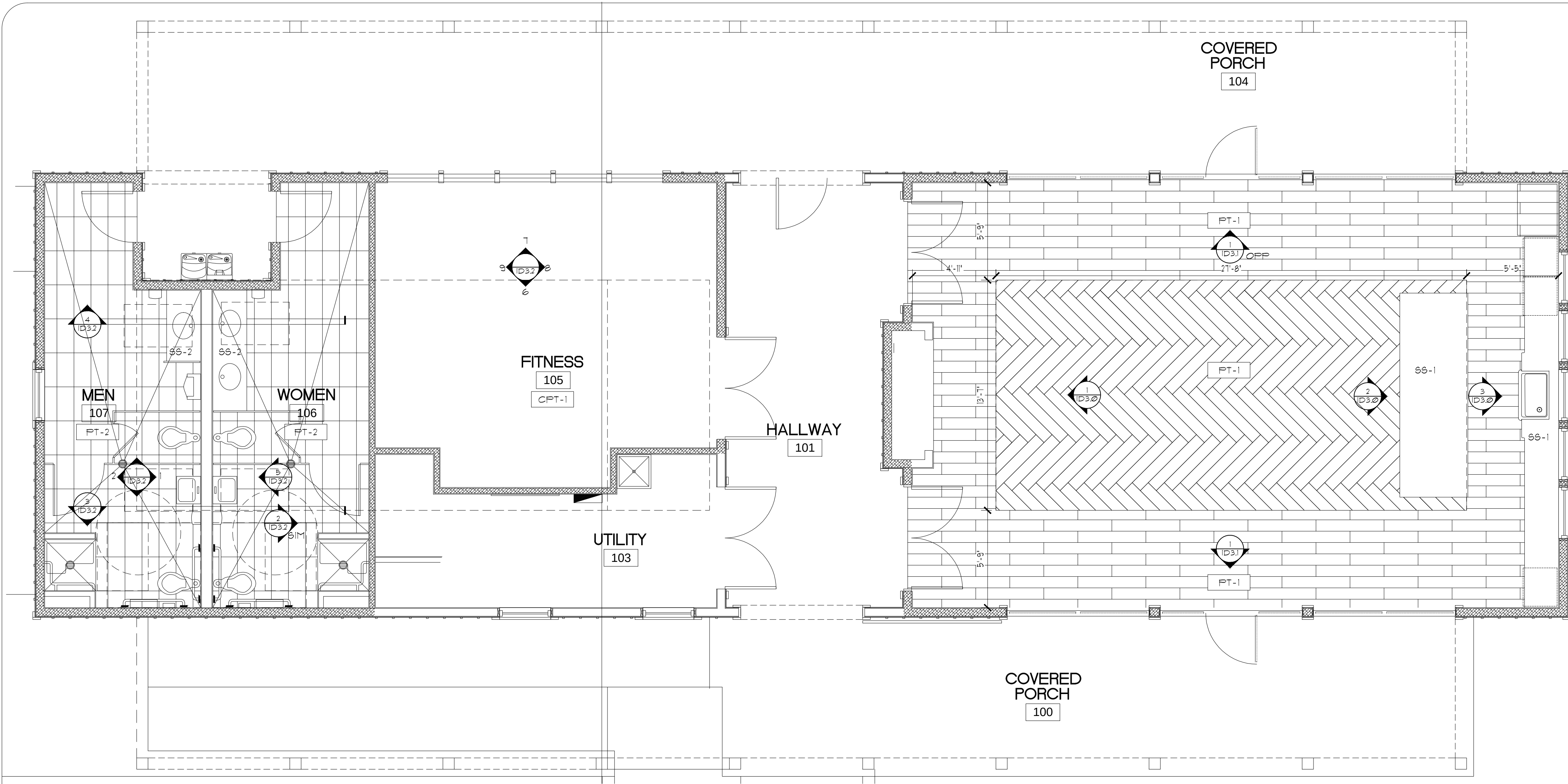
1 INTERIOR FLOOR PLAN
