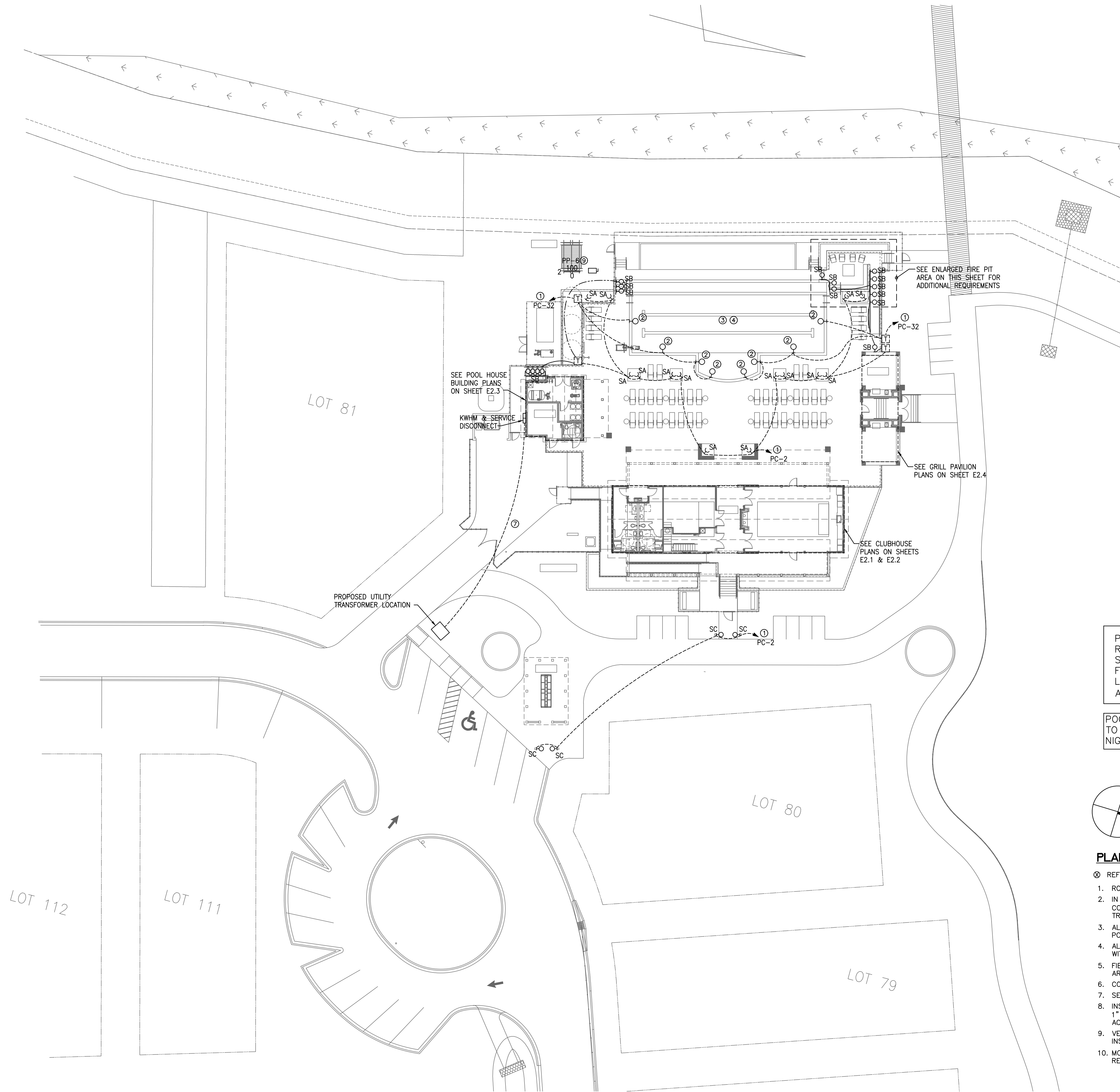
ELECTRICAL SITE PLAN SCALE 1"=20'-0"
