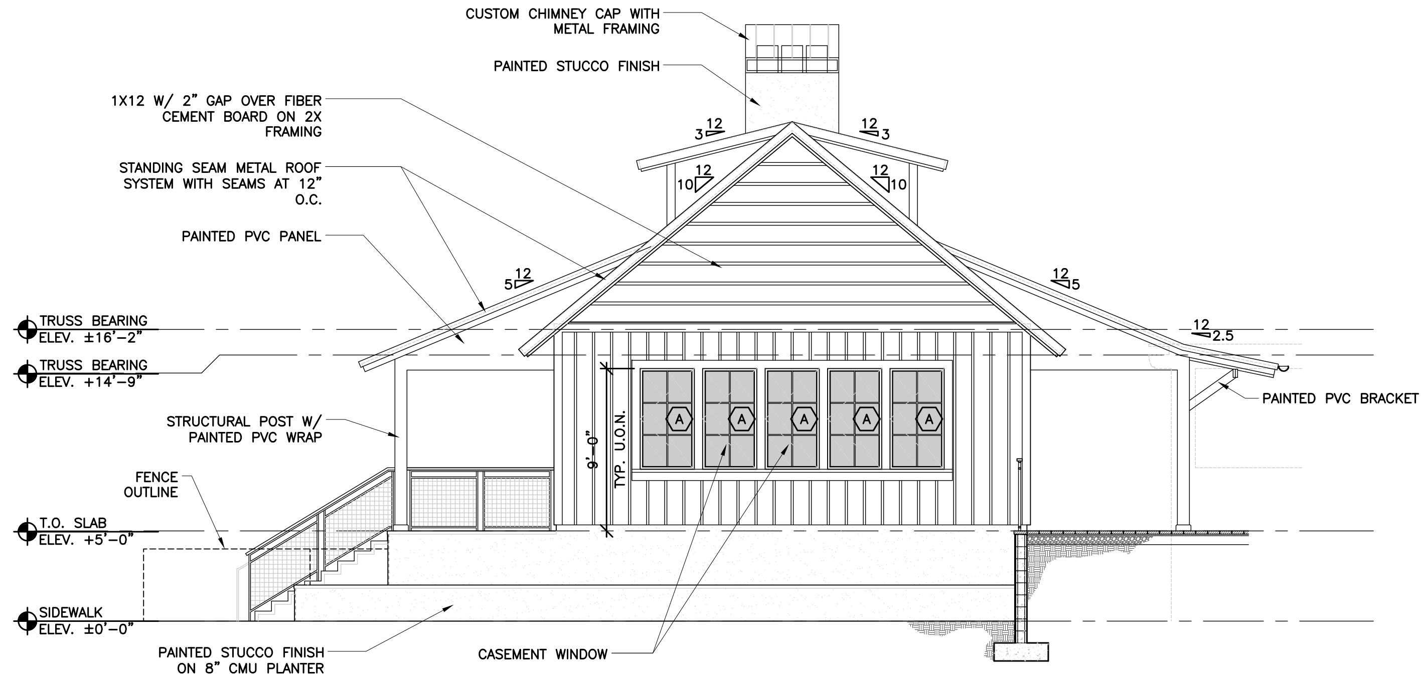
3 CLUBHOUSE LEFT SIDE ELEVATION SCALE: 3/16"=1'-0"
