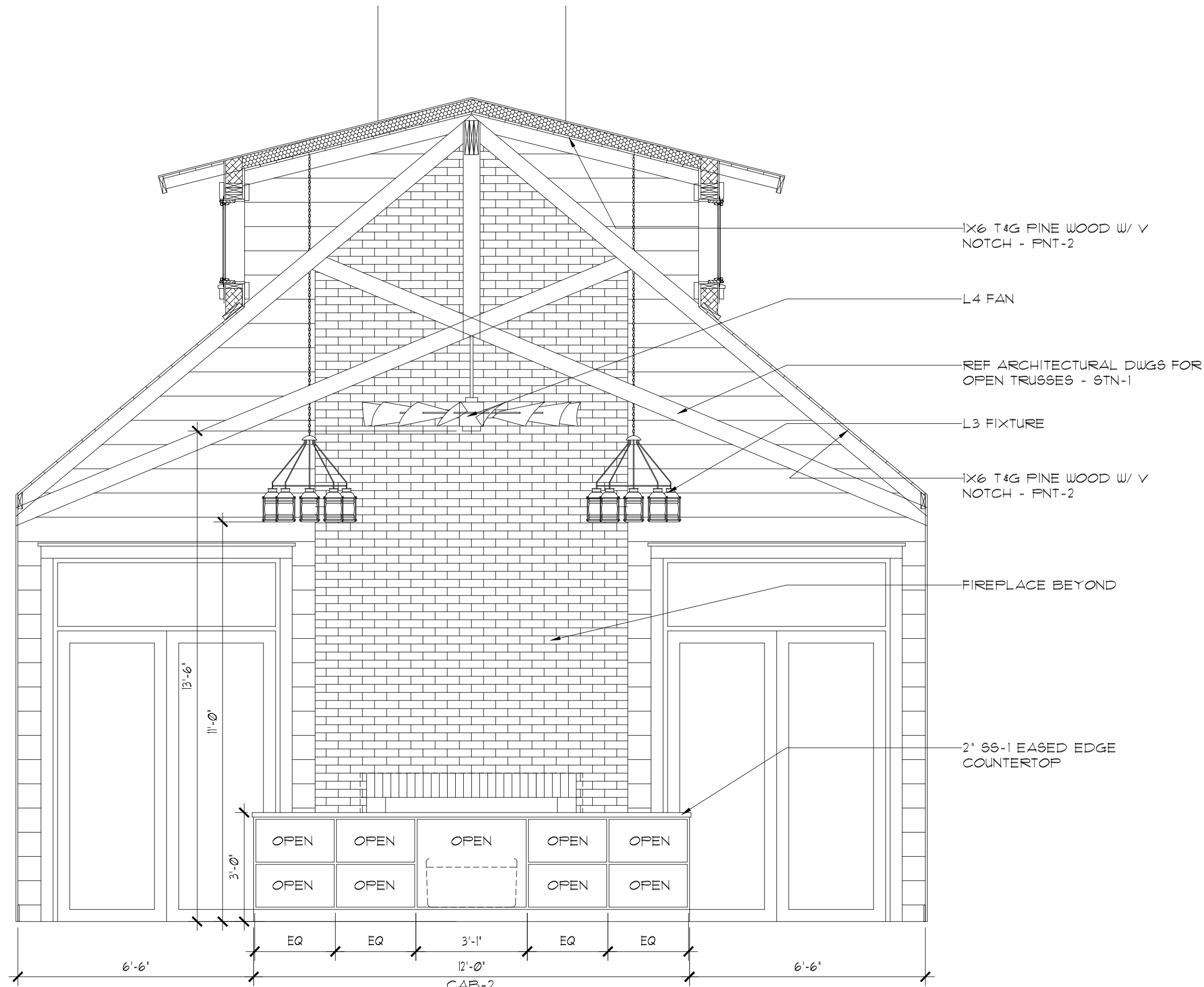
2 RM 102 - EAST WALL SCALE: 3/8" = 1'-0"
