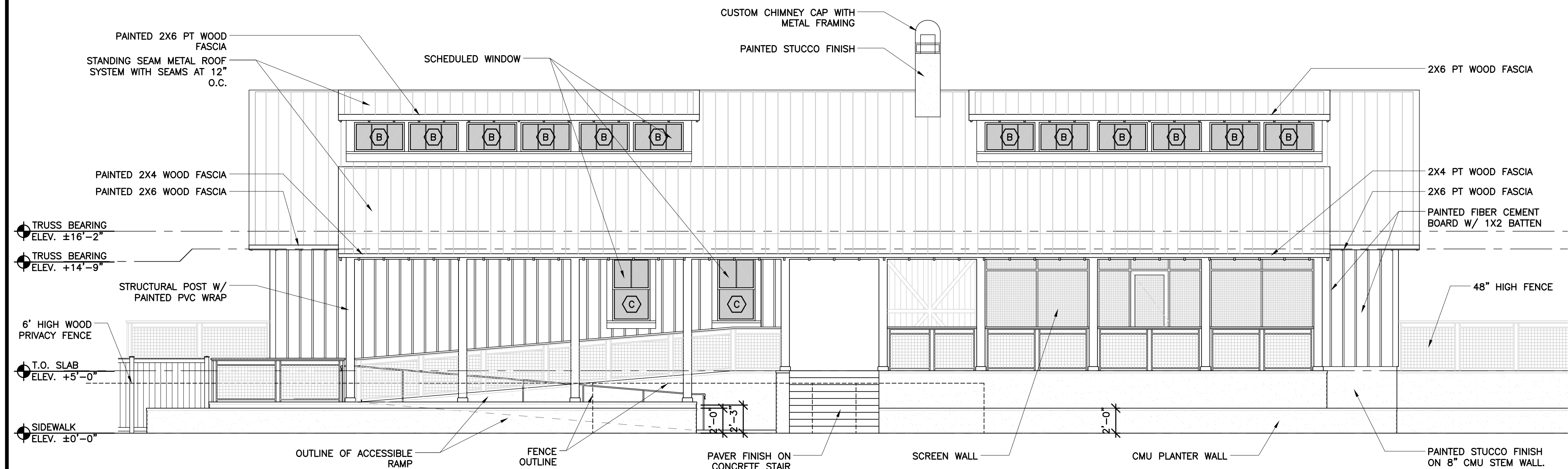
1 CLUBHOUSE ENTRY ELEVATION SCALE: 3/16"=1'-0"
