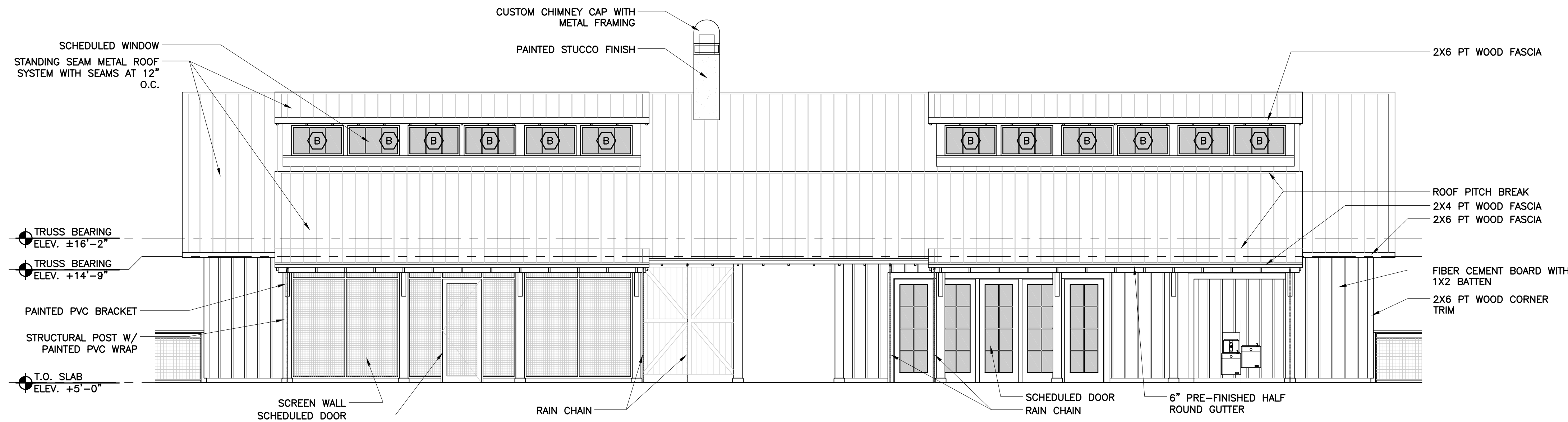
1 CLUBHOUSE POOL ELEVATION SCALE: 3/16"=1'-0"
